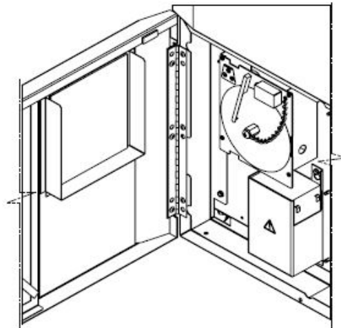
Figure 71. Chart Recorder
